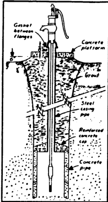
Figure 6: Dug Well Constructed with a Buried Slab
